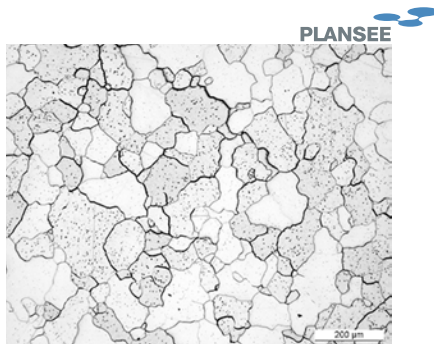
Coarse grain-structure for best creep-resistance
