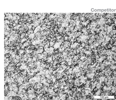
Fine grain-structure with low creep-resistance
